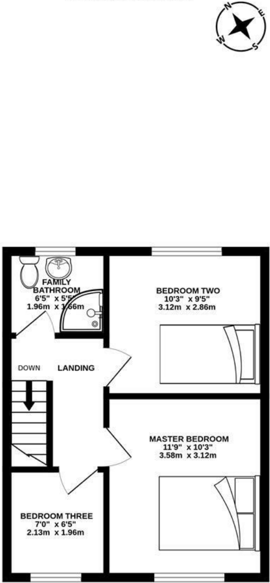
1ST FLOOR 352 sq.ft. (32.7 sq.m.) approx.
